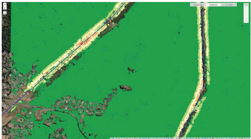
Figure 2. From LiDAR, data risk of arcing is interpolated. 3D viewing provides context and verification.
