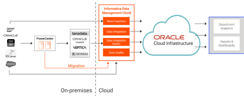
Figure 1. Cloud Data Management Reference Architecture.
