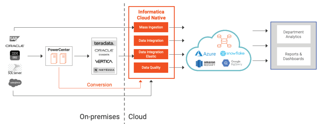
Figure 1. Cloud Data Management Reference Architecture.
